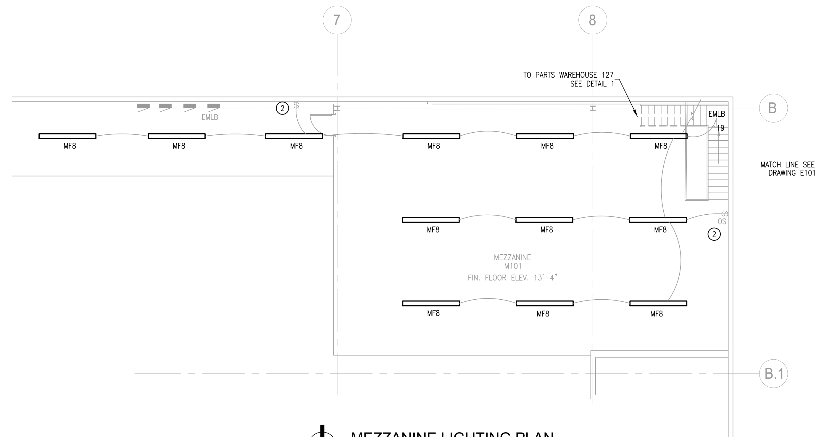
MEZZANINE LIGHTING PLAN
