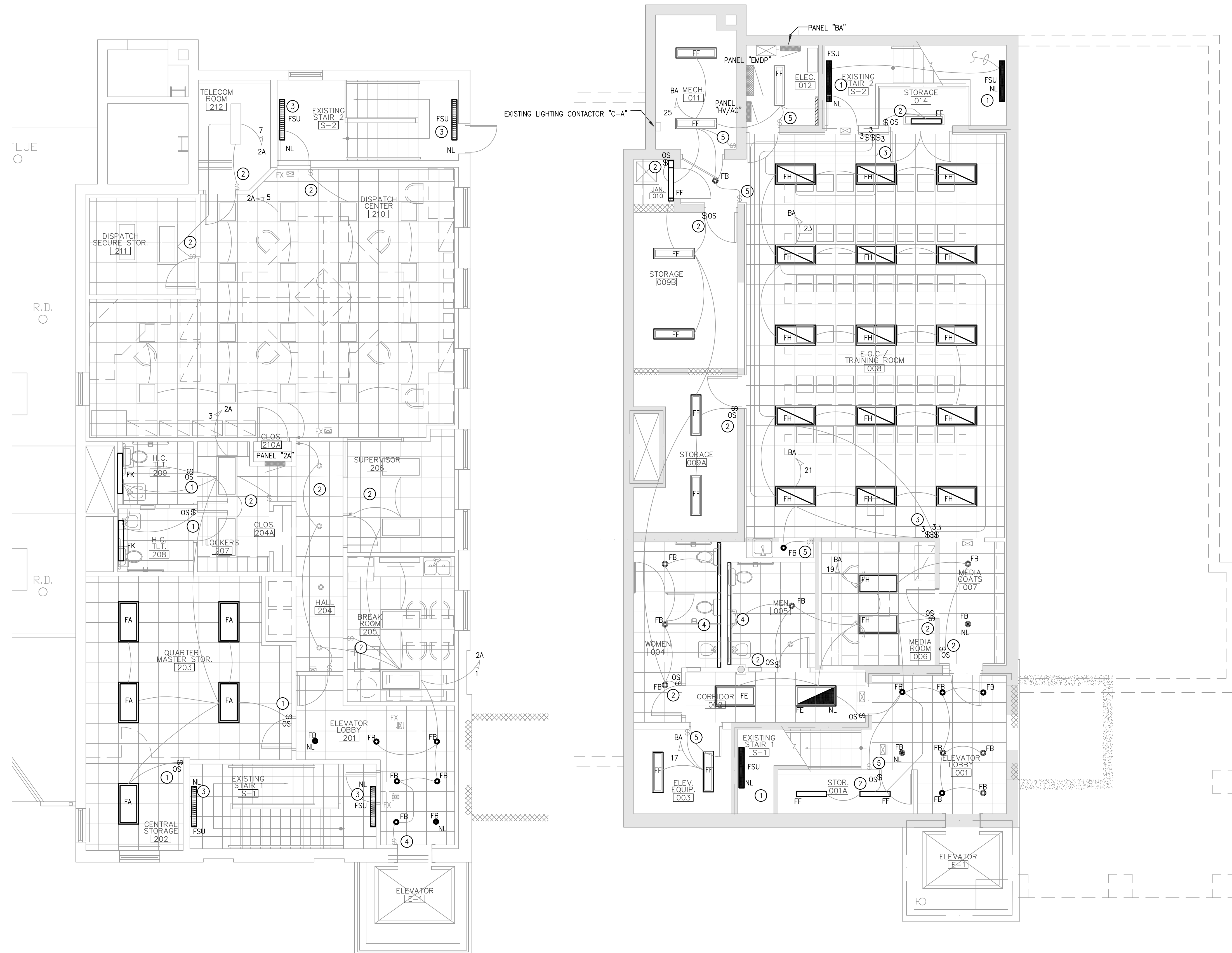
DISPATCH SECOND LEVEL LIGHTING PLAN SCALE 3/16" = 1'0"
