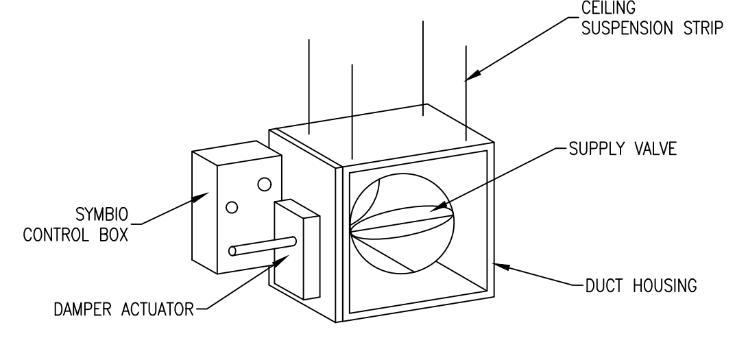
4 ZONE DAMPER DETAIL
