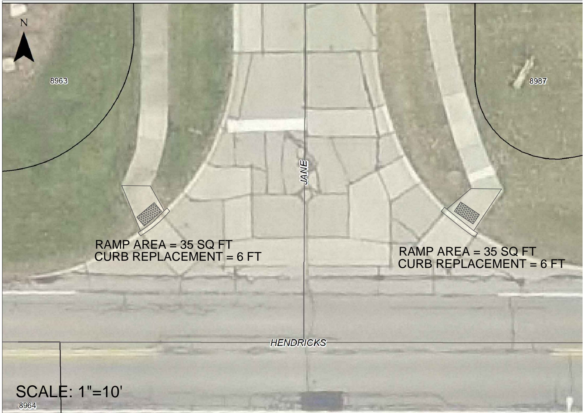
RAMP REPLACEMENT AT HENDRICKS RD. & JANE DR.
