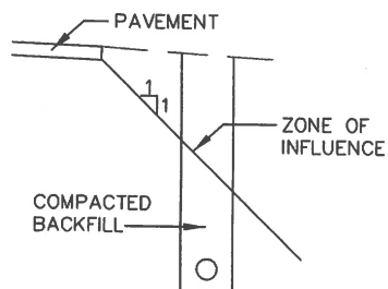
PARALLEL ZONE OF INFLUENCE
