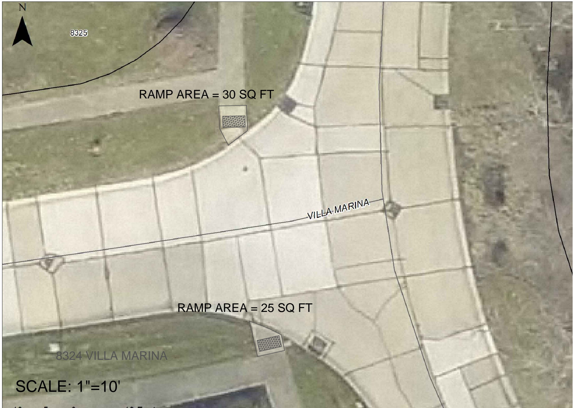
RAMP REPLACEMENT AT 8324 & 8325 VILLA MARINA
