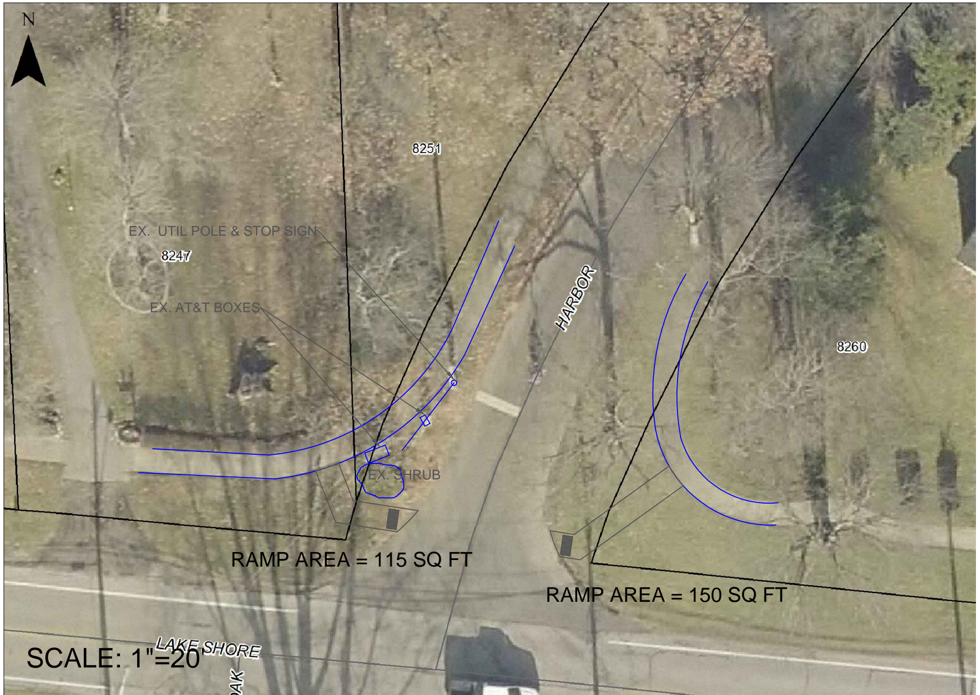
NEW RAMP CONSTRUCTION AT HARBOR DR & LAKESHORE BLVD.
