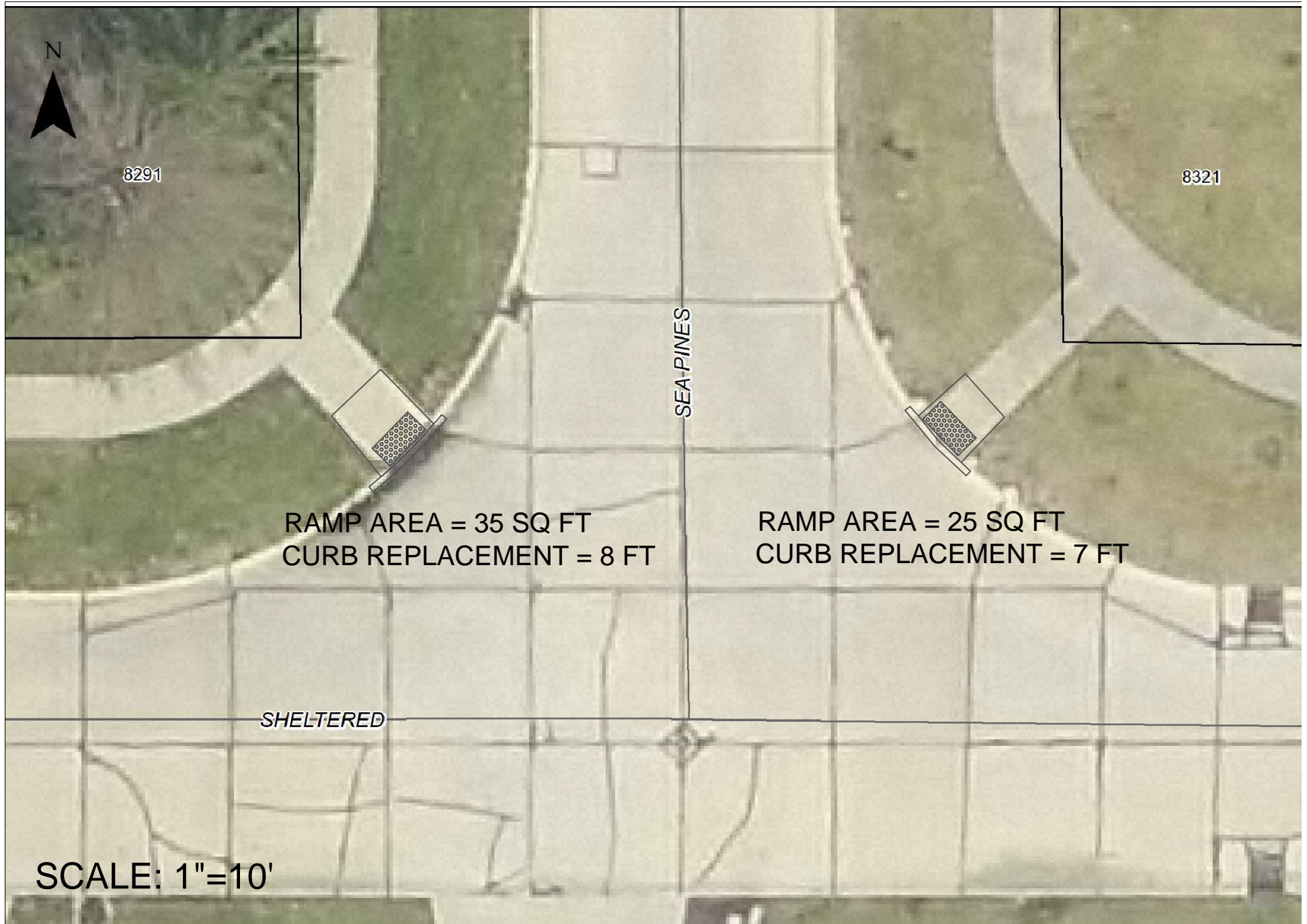
RAMP REPLACEMENT AT SEA PINES & SHELTERED COVE
