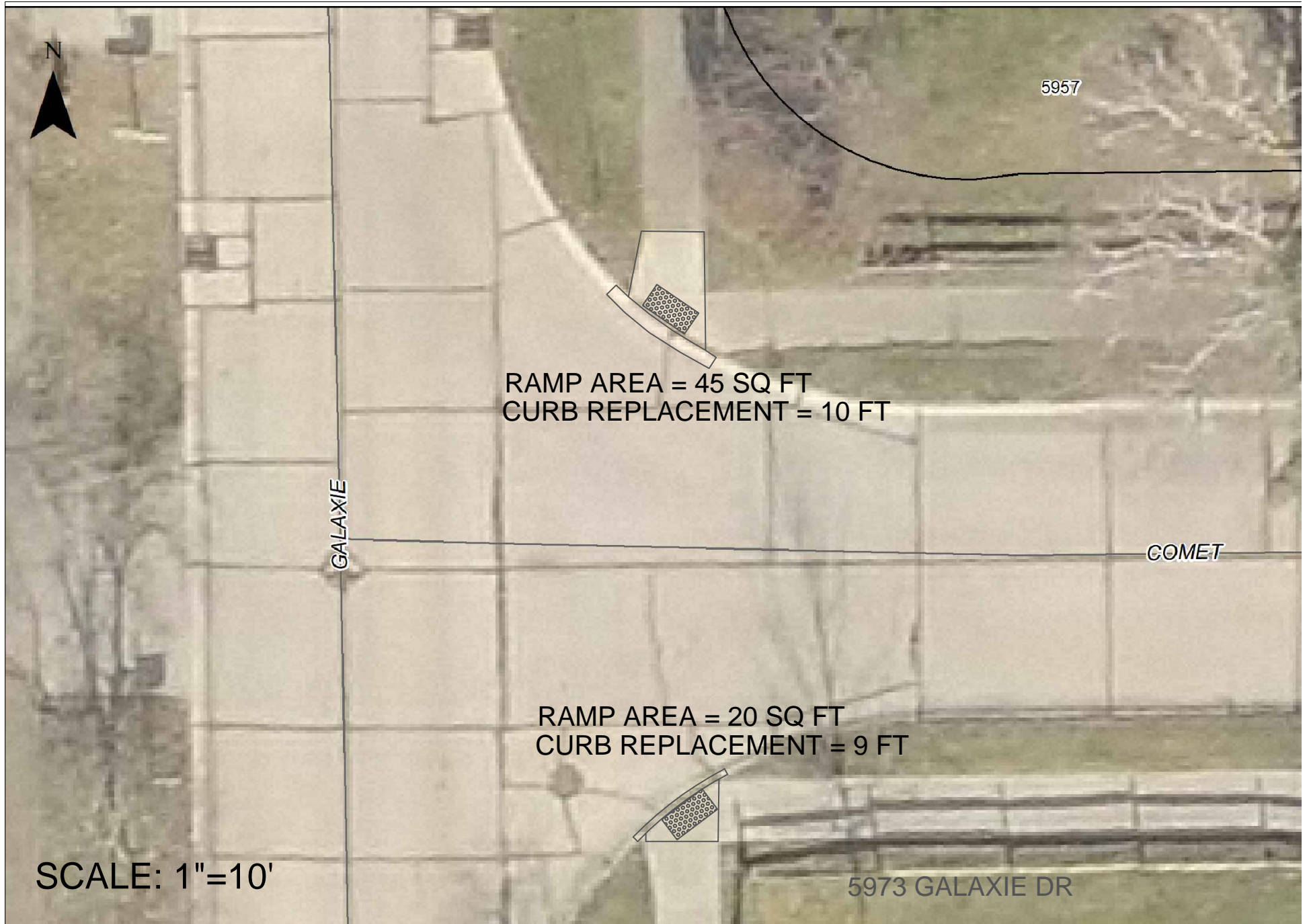
RAMP REPLACEMENT AT GALAXIE DR. & COMET CT.
