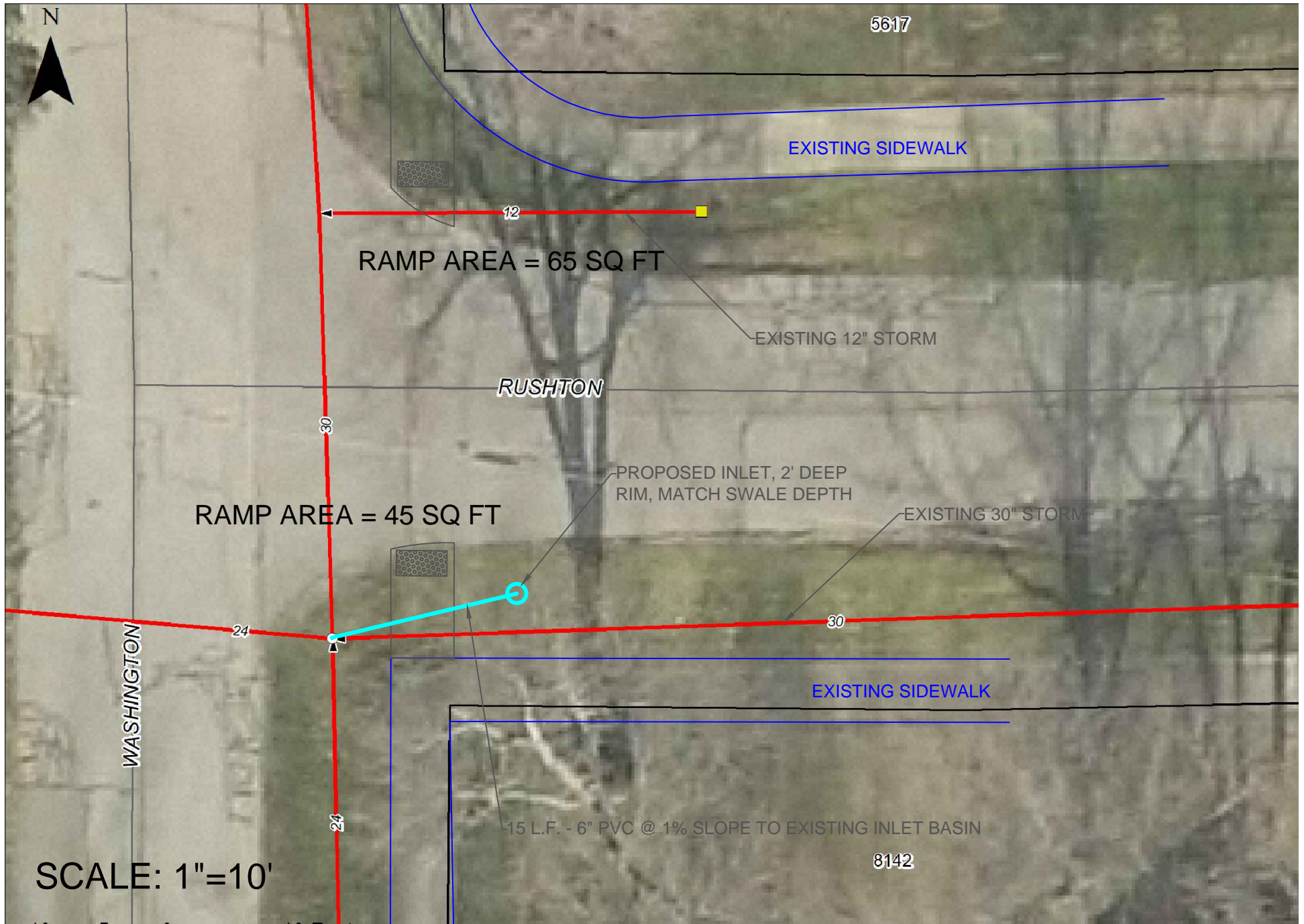
NEW RAMP CONSTRUCTION AT RUSHTON DR. & WASHINGTON AVE.
