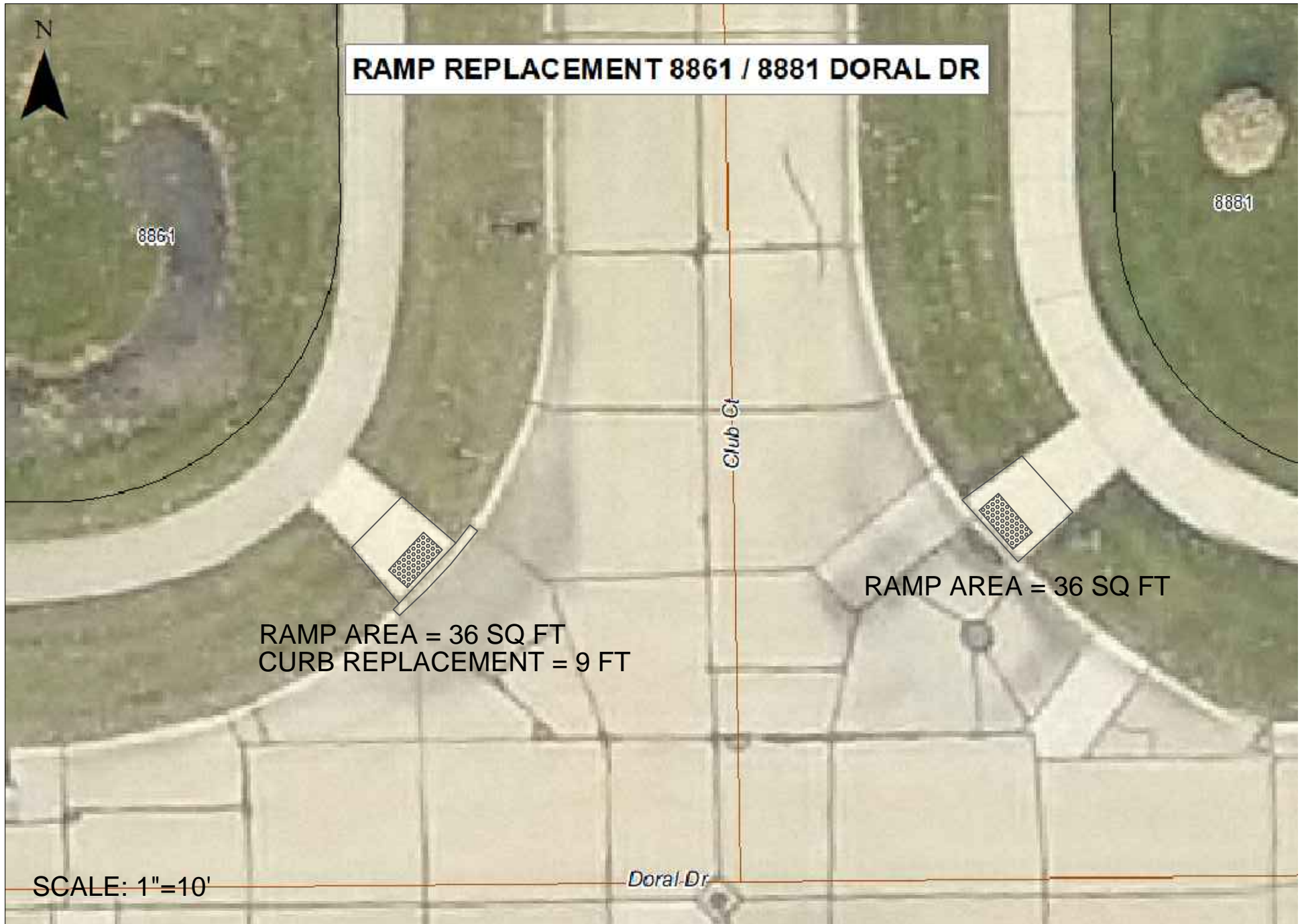
RAMP REPLACEMENT AT DORAL DR. & CLUB CT.
