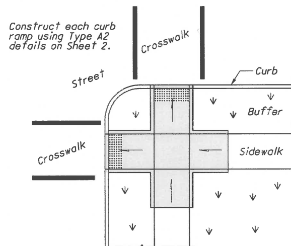
PERPENDICULAR CURB RAMPS
