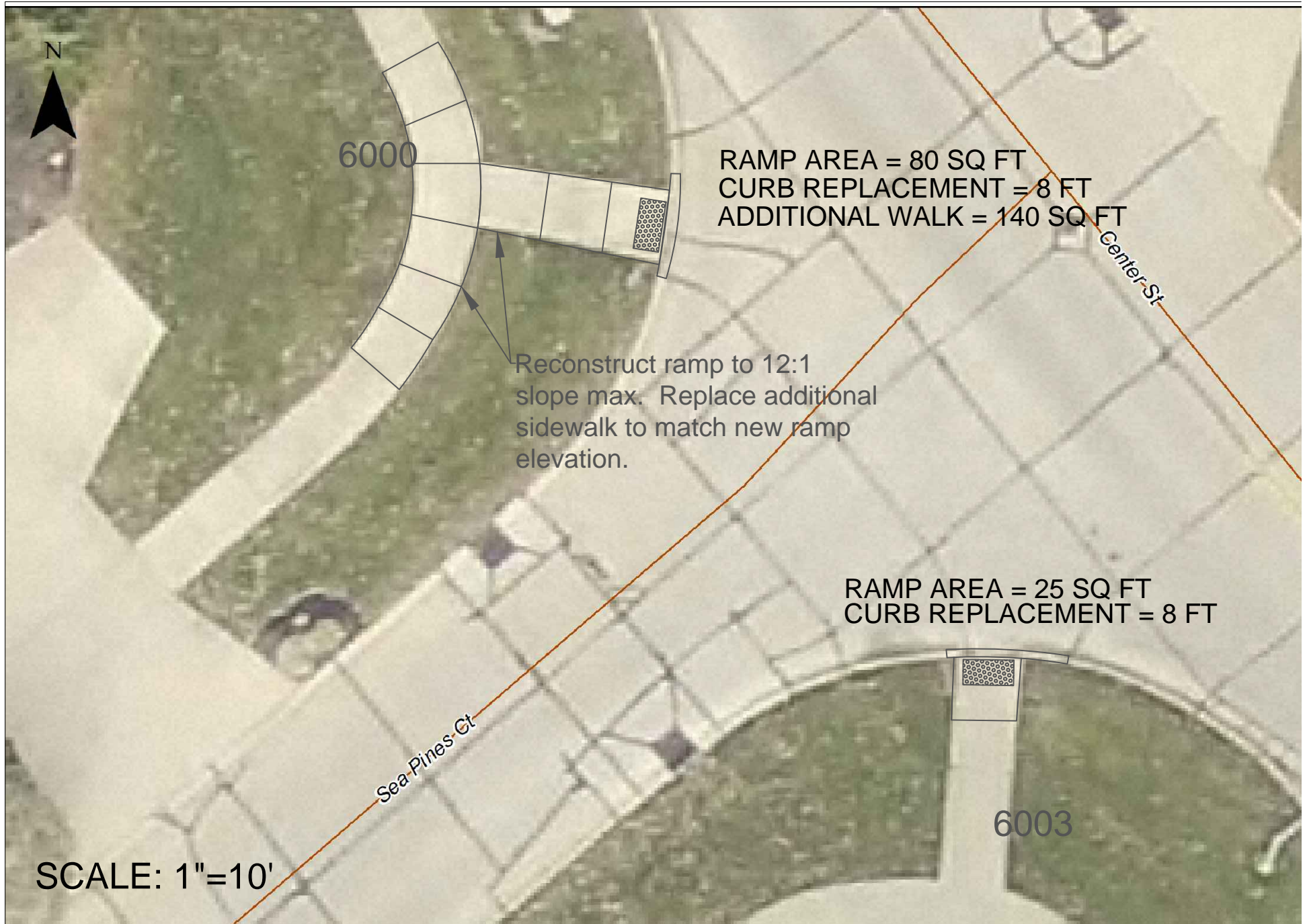
RAMP REPLACEMENT AT CENTER ST. & SEA PINES CT.
