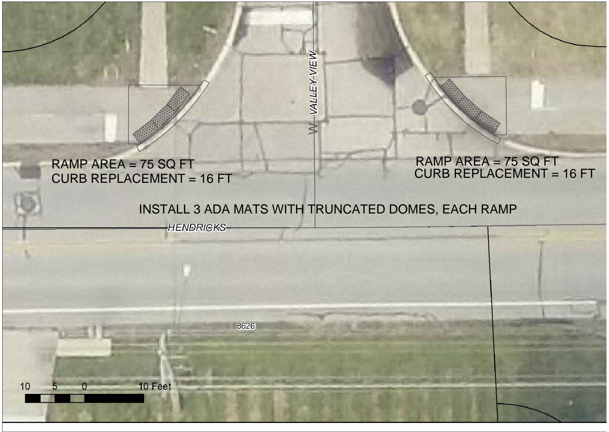
RAMP REPLACEMENT AT HENDRICKS RD. & W. VALLEY VIEW
