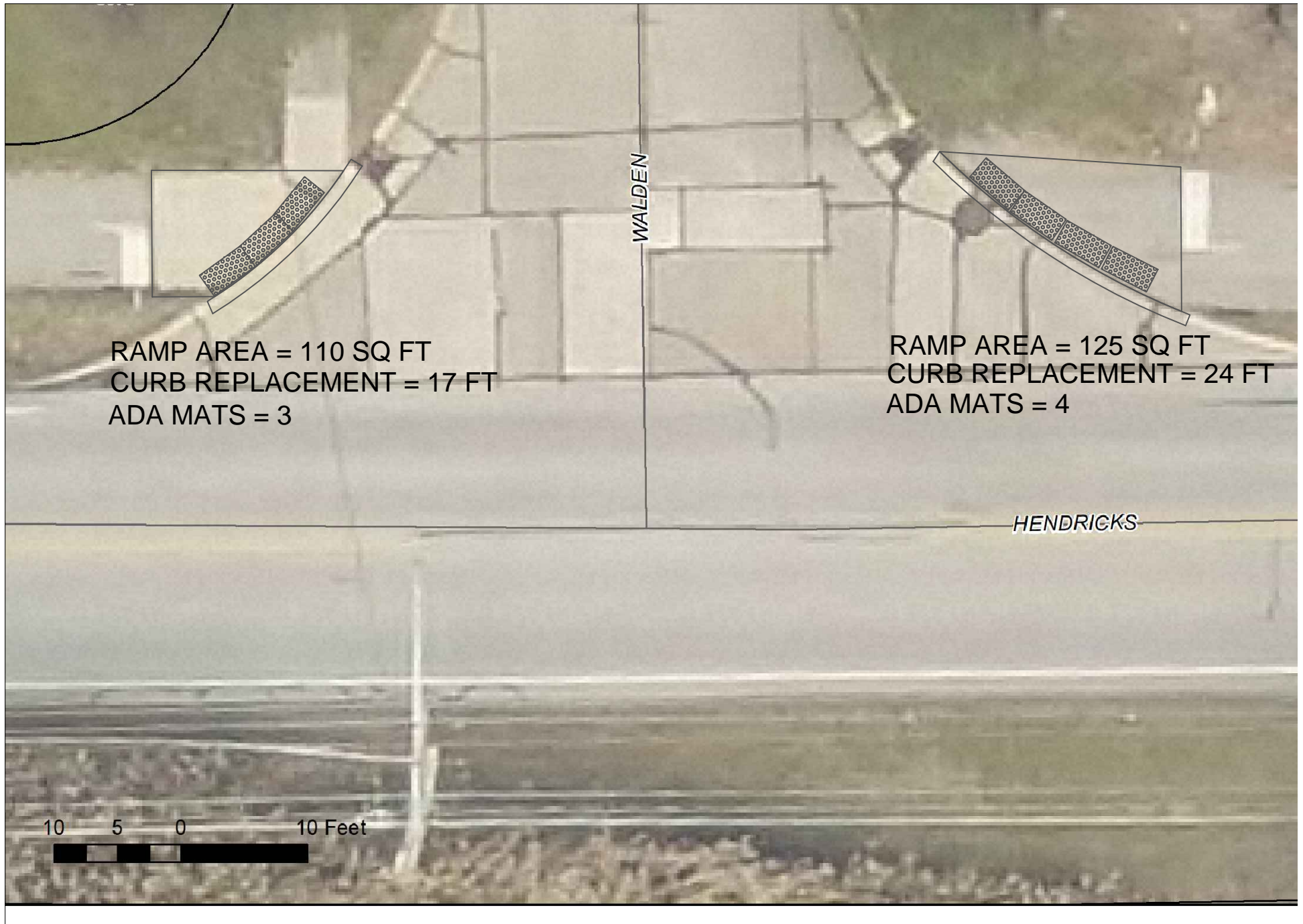
RAMP REPLACEMENT AT HENDRICKS RD. & WALDEN CT.
