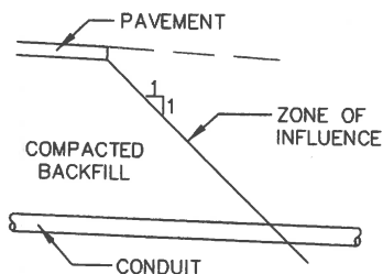
TRANSVERSE ZONE OF INFLUENCE
