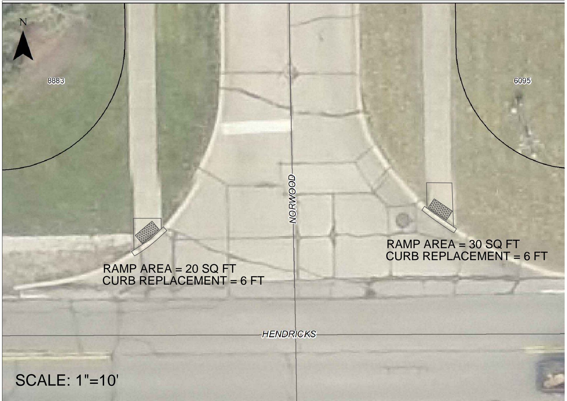
RAMP REPLACEMENT AT HENDRICKS RD. & NORWOOD DR.
