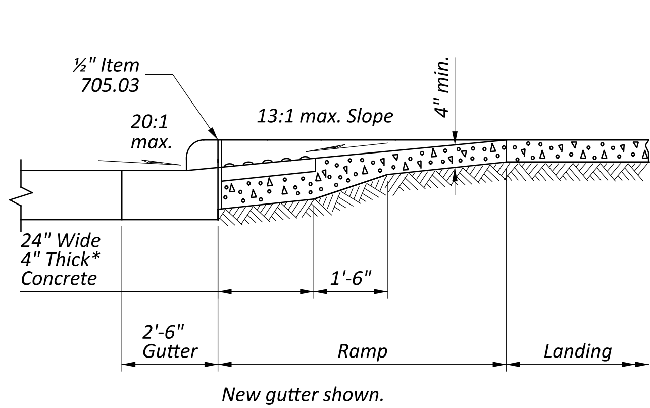
SECTION A-A NORMAL DETAIL
