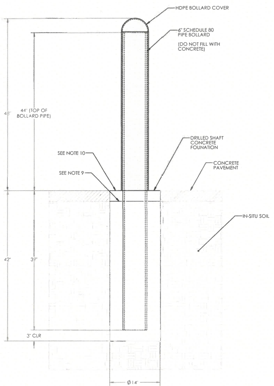
DEEP MOUNT S20 BOLLARD IN CONCRETE PAVING
