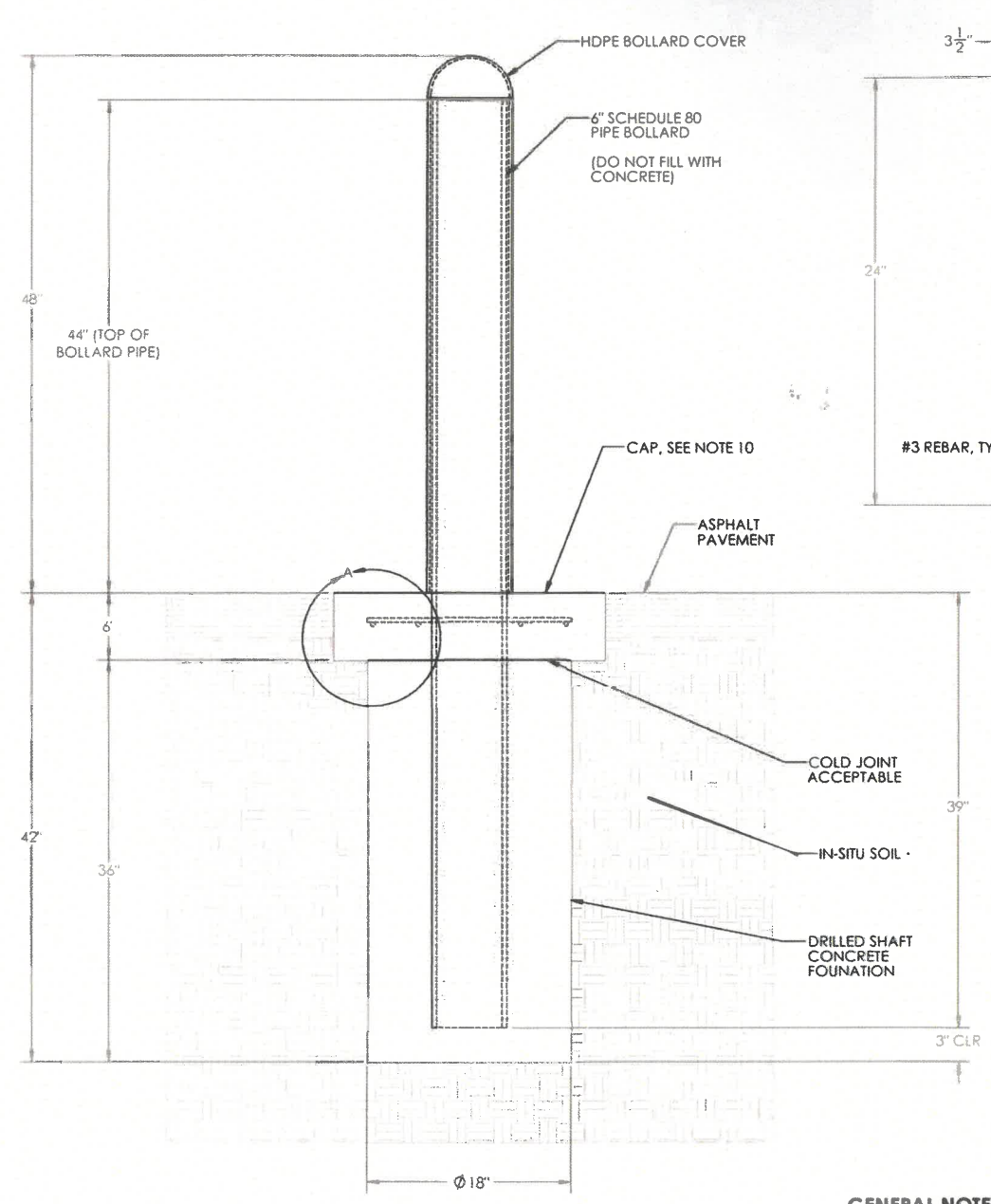
DEEP MOUNT S20 BOLLARD IN ASPHALT PAVING
