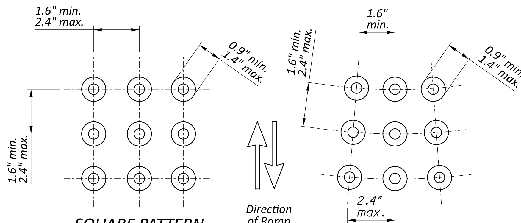
RADIAL ALIGNMENT
