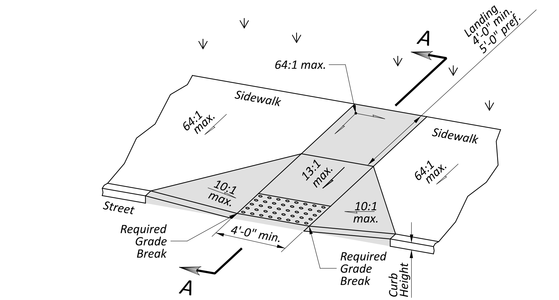
Type A1 (Perpendicular with flared sides)
