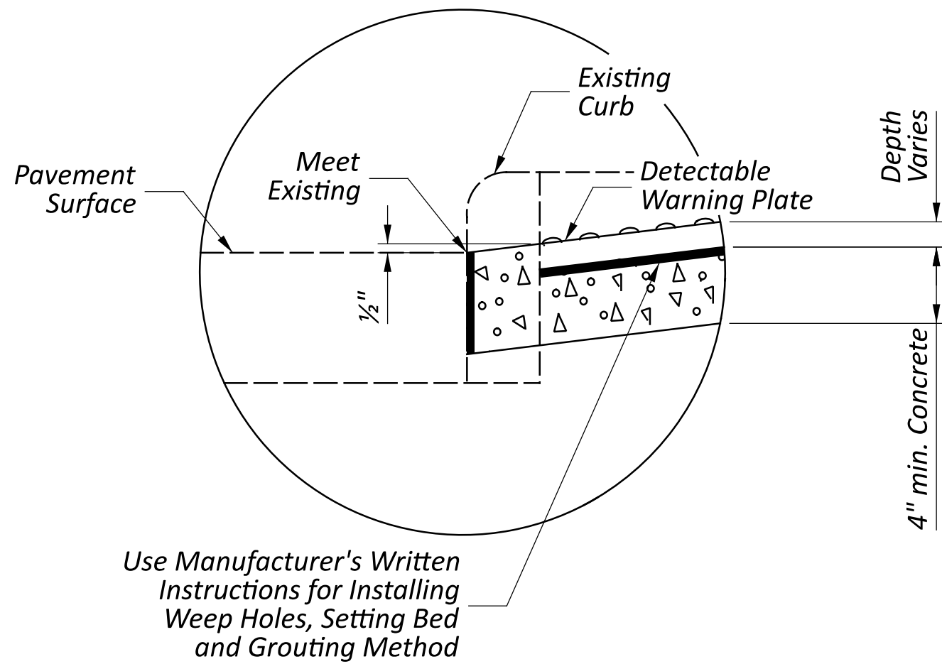
DETAIL A
