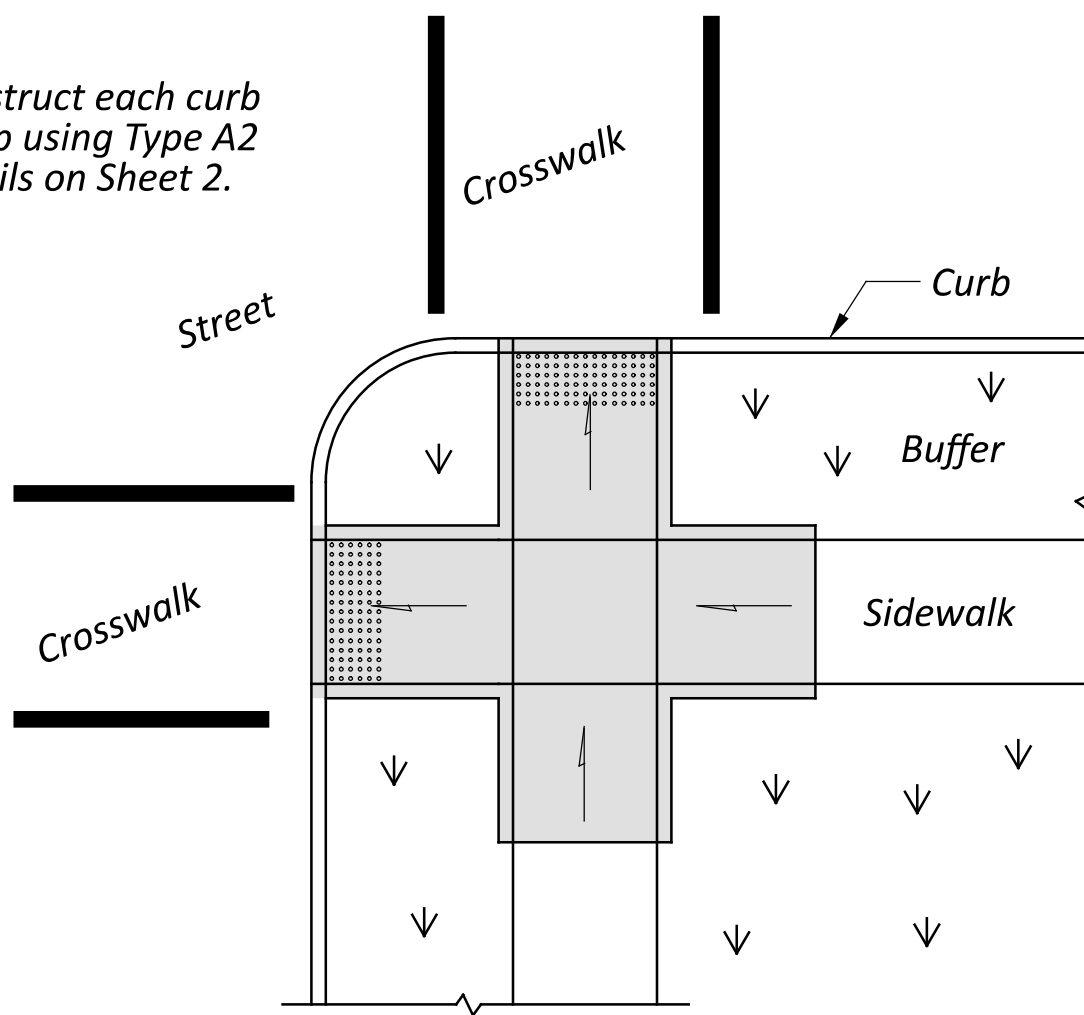
PERPENDICULAR CURB RAMPS
