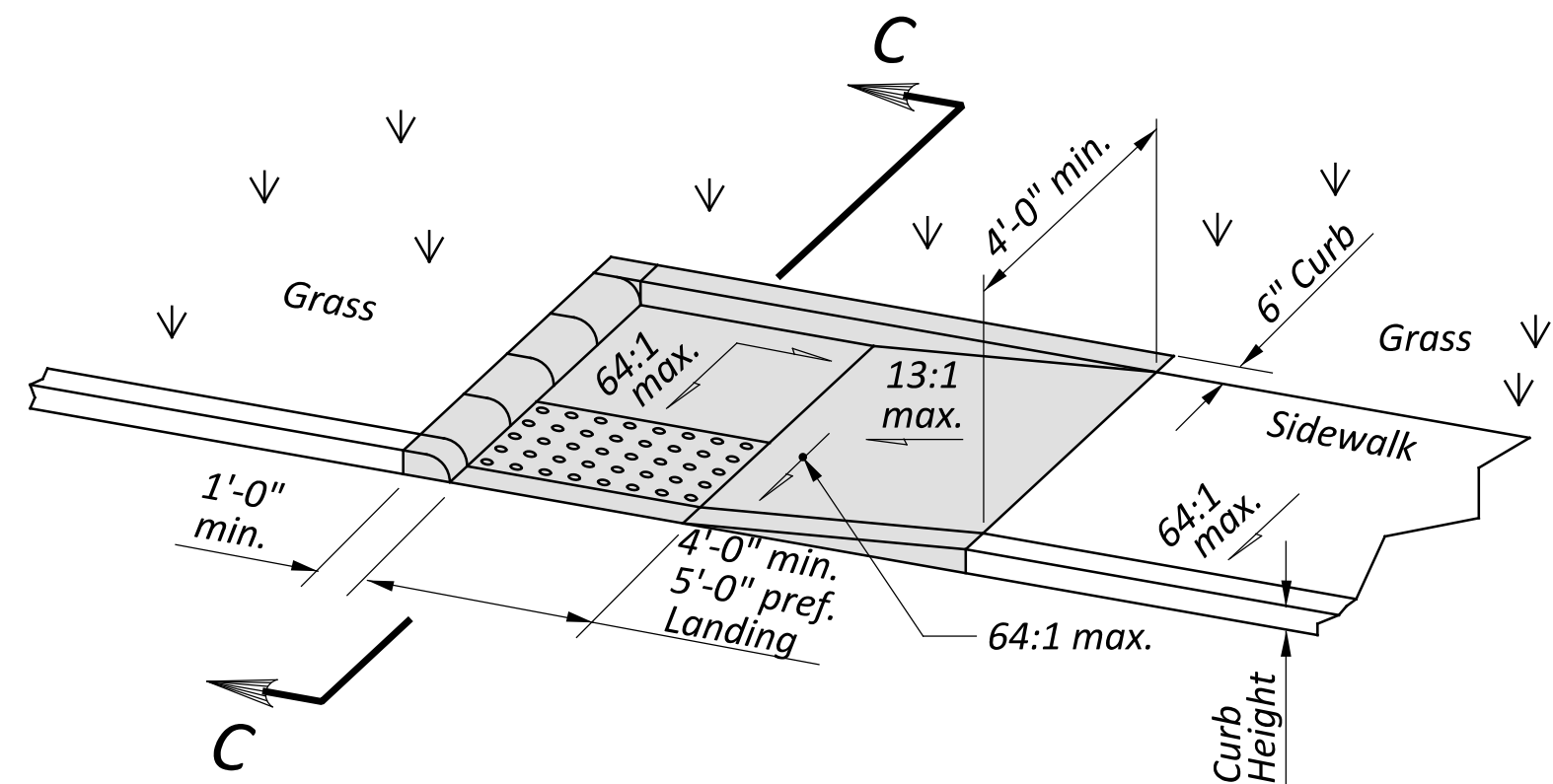
Type B1 (Single sided Parallel)
