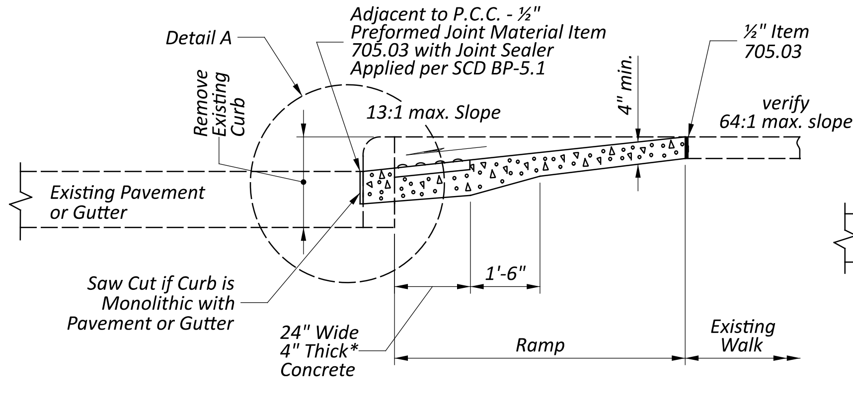
SECTION A-A EXISTING WALK DETAIL
