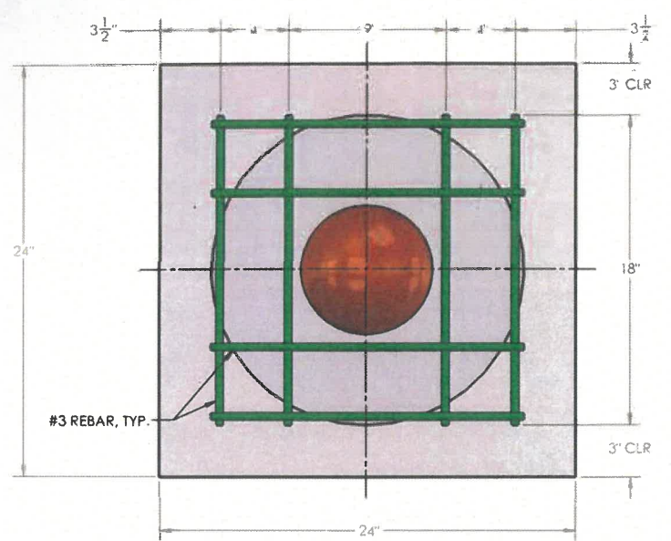
CAP REINFORCING DETAILS
