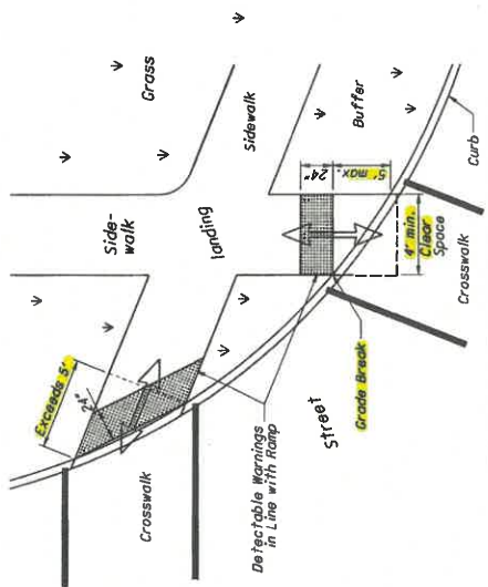
DETECTABLE WARNING ALIGNMENT
