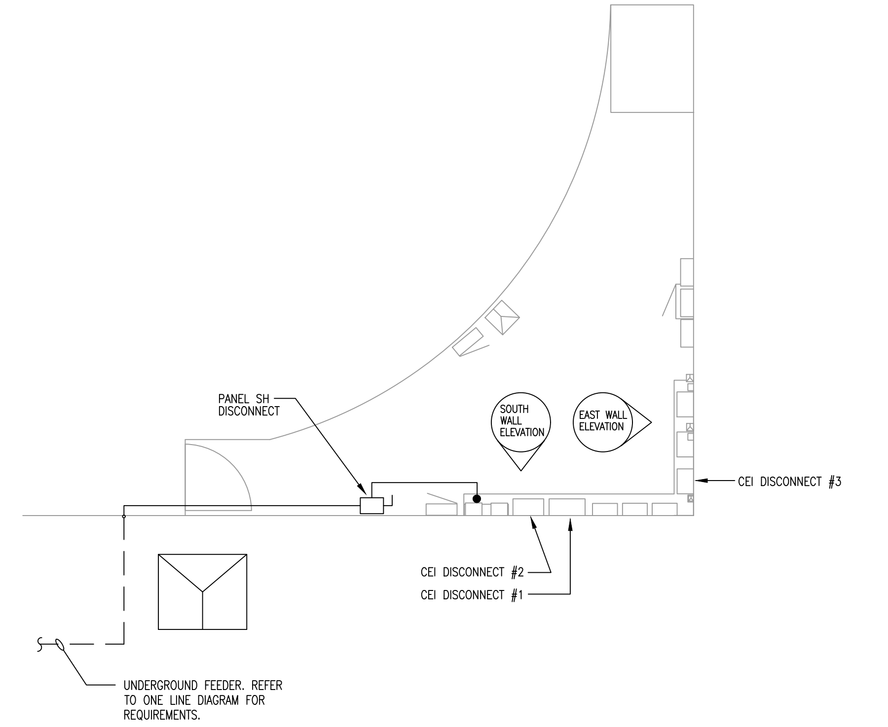
MAIN ELECTRICAL ROOM PLAN Scale: 1/4" = 1'0"
